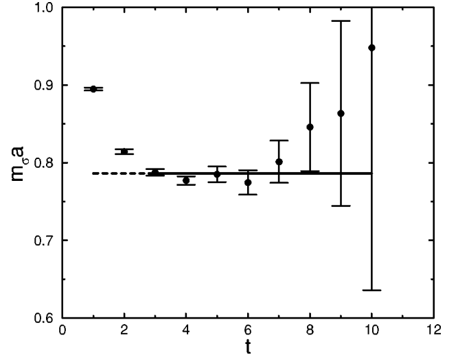
FIG. 13. Scalar effective masses and fitted mass for \beta of 5.93 and \kappa of 0.1567 on a lattice 24^4 .
