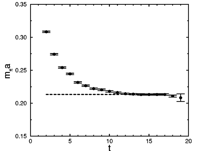
FIG. 6. Pseudoscalar effective masses and fitted mass for \beta of 6.40 and \kappa of 0.1491 on a lattice 32^2 \times 28 \times 40 .
