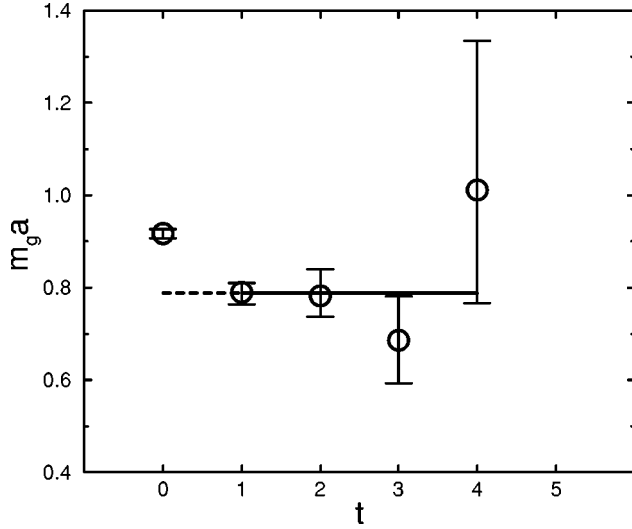
FIG. 27. Scalar glueball effective masses and fitted mass for \beta of 5.93 on a lattice 16^2 \times 14 \times 20 .
