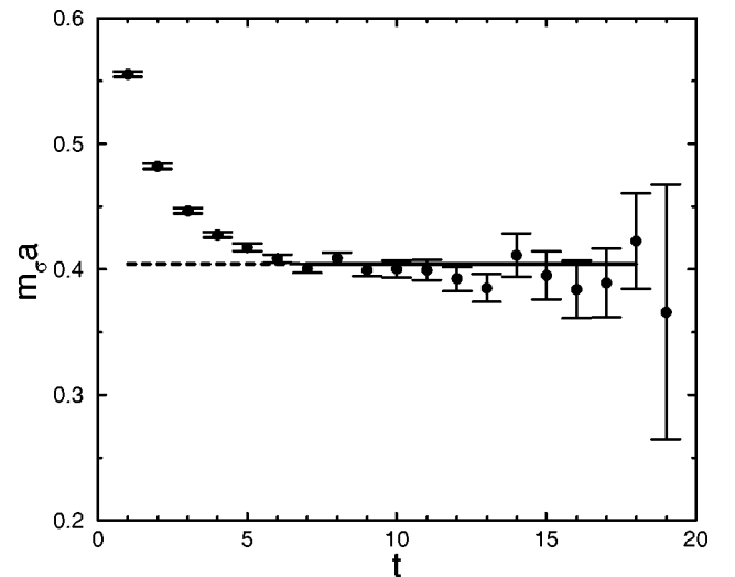
FIG. 14. Scalar effective masses and fitted mass for \beta of 6.40 and \kappa of 0.1491 on a lattice 32^2 \times 28 \times 40 .
