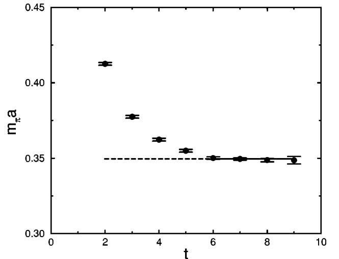
FIG. 2. Pseudoscalar effective masses and fitted mass for \beta of 5.93 and \kappa of 0.1562 on a lattice 16^2 \times 14 \times 20 .
