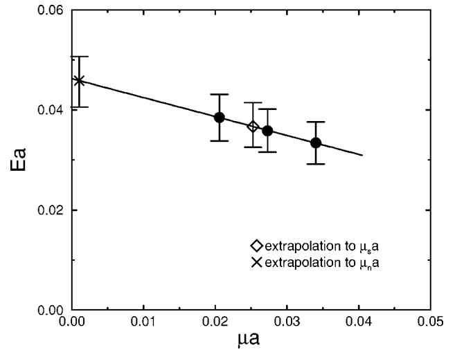
FIG. 42. Glueball-quarkonium mixing energy as a function of quark mass for \beta of 6.40.
