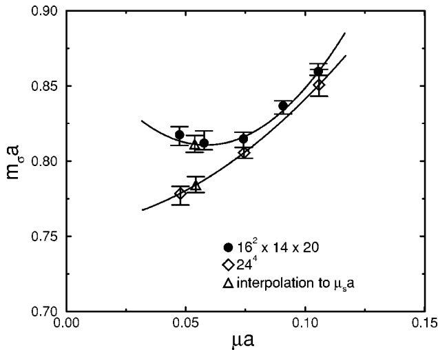
FIG. 21. Scalar quarkonium mass as a function of quark mass for \beta of 5.93.
