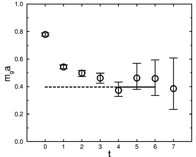
FIG. 30. Scalar glueball effective masses and fitted mass for \beta of 6.40 on a lattice 32^2 \times 28 \times 40 .
