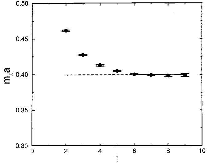
FIG. 1. Pseudoscalar effective masses and fitted mass for \beta of 5.93 and \kappa of 0.1554 on a lattice 16^2 \times 14 \times 20 .
