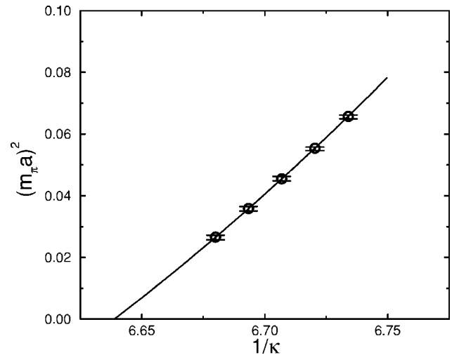
FIG. 20. Pseudoscalar quarkonium mass squared as a function of 1/\kappa for \beta of 6.4 on the lattice 32^2 \times 28 \times 40 .
