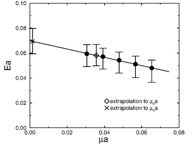
FIG. 41. Glueball-quarkonium mixing energy as a function of quark mass for \beta of 6.17.
