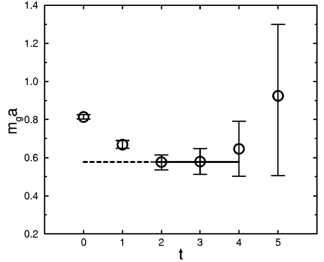
FIG. 29. Scalar glueball effective masses and fitted mass for \beta of 6.17 on a lattice 24^2 \times 20 \times 32 .
