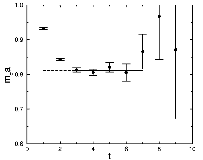
FIG. 10. Scalar effective masses and fitted mass for \beta of 5.93 and \kappa of 0.1562 on a lattice 16^2 \times 14 \times 20 .
