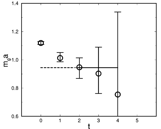
FIG. 26. Scalar glueball effective masses and fitted mass for \beta of 5.70 on a lattice 12^2 \times 10 \times 24 .
