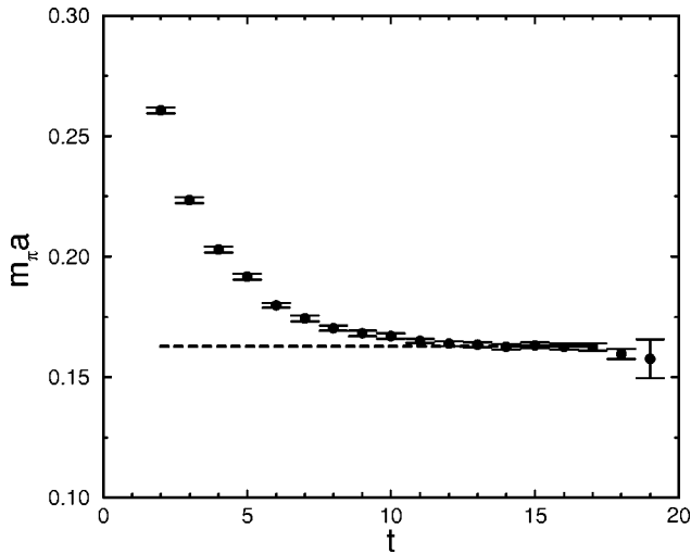
FIG. 8. Pseudoscalar effective masses and fitted mass for \beta of 6.40 and \kappa of 0.1497 on a lattice 32^2 \times 28 \times 40 .
