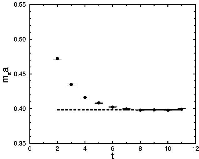
FIG. 4. Pseudoscalar effective masses and fitted mass for \beta of 5.93 and \kappa of 0.1554 on a lattice 24^4 .
