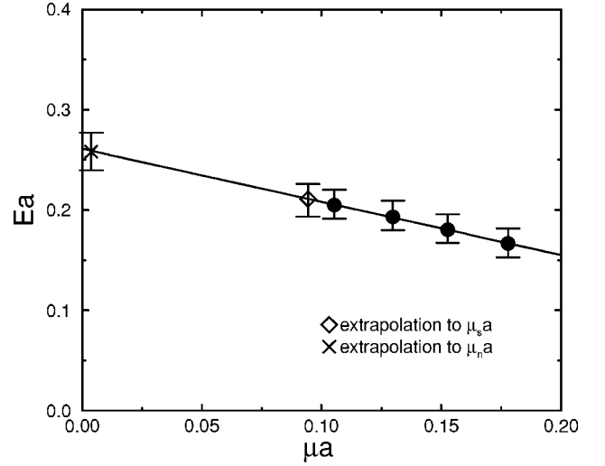
FIG. 40. Glueball-quarkonium mixing energy as a function of quark mass for \beta of 5.70.
