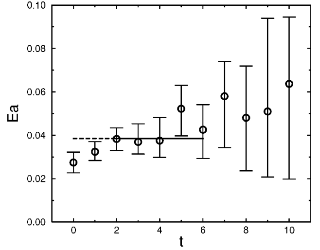
FIG. 38. Effective mixing energy and fitted mixing energy for \beta of 6.40 and \kappa of 0.1497 on a lattice 32^2 \times 28 \times 40 .
