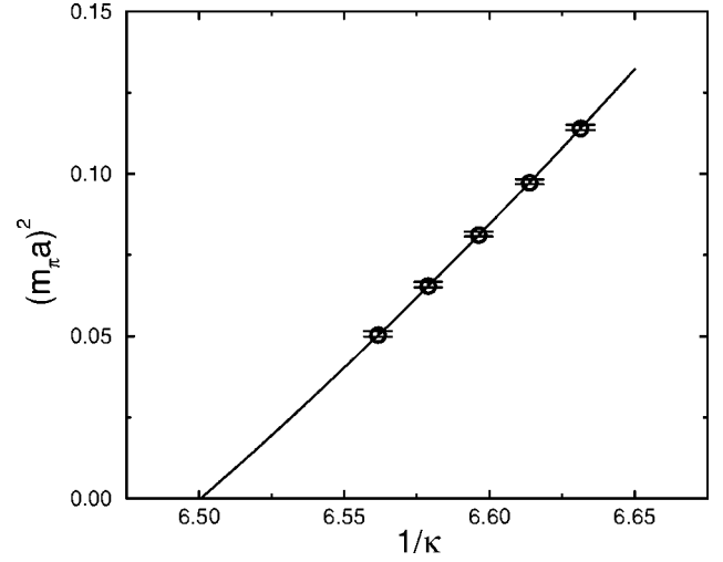
FIG. 19. Pseudoscalar quarkonium mass squared as a function of 1/\kappa for \beta of 6.17 on the lattice 24^2 \times 20 \times 32 .
