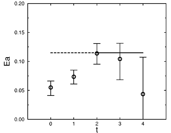
FIG. 34. Effective mixing energy and fitted mixing energy for \beta of 5.93 and \kappa of 0.1554 on a lattice 24^4 .
