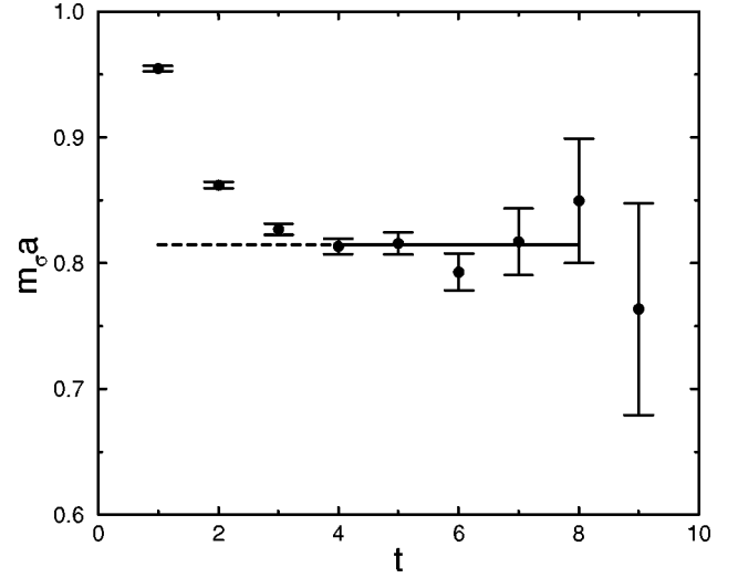
FIG. 9. Scalar effective masses and fitted mass for \beta of 5.93 and \kappa of 0.1554 on a lattice 16^2 \times 14 \times 20 .
