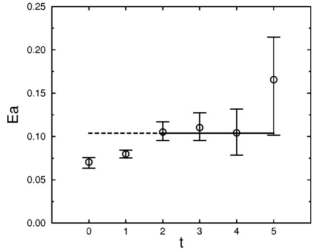
FIG. 33. Effective mixing energy and fitted mixing energy for \beta of 5.93 and \kappa of 0.1567 on a lattice 16^2 \times 14 \times 20 .
