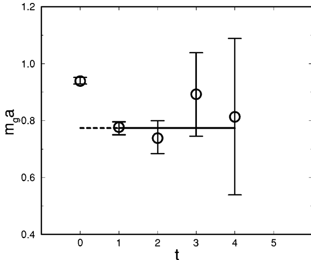
FIG. 28. Scalar glueball effective masses and fitted mass for \beta of 5.93 on a lattice 24^4 .
