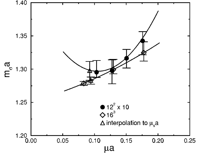
FIG. 22. Scalar quarkonium mass as a function of quark mass for \beta of 5.7.
